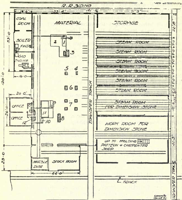
FIG. 101—PLAN AND LAYOUT OF PLANT NO. 2
